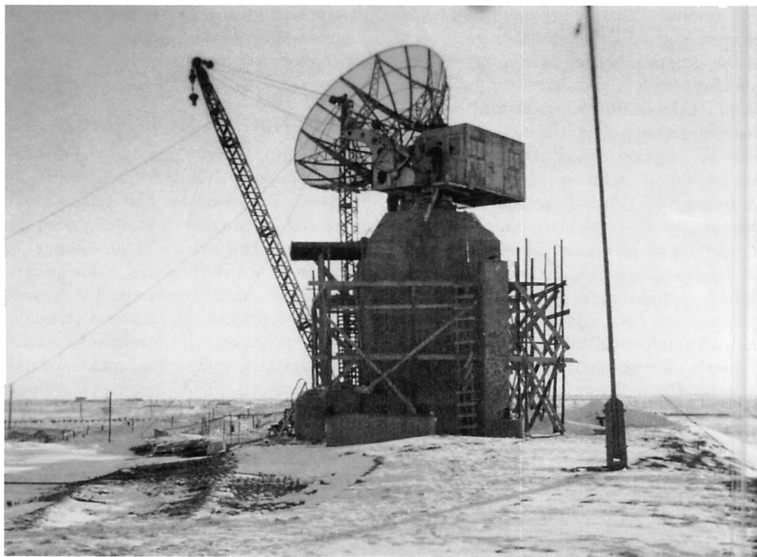
Radar under montering i 1944.
