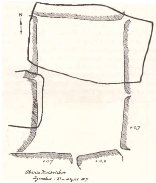
Diagram over Dyssestuen: Dysse Nr. 7
